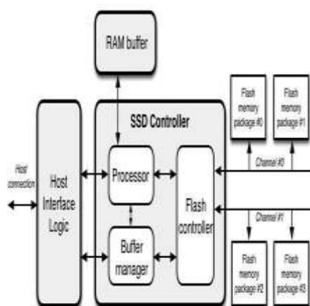
Fig 1 SSD Block Diagram
